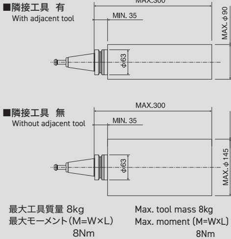
Maximum tool dimension
